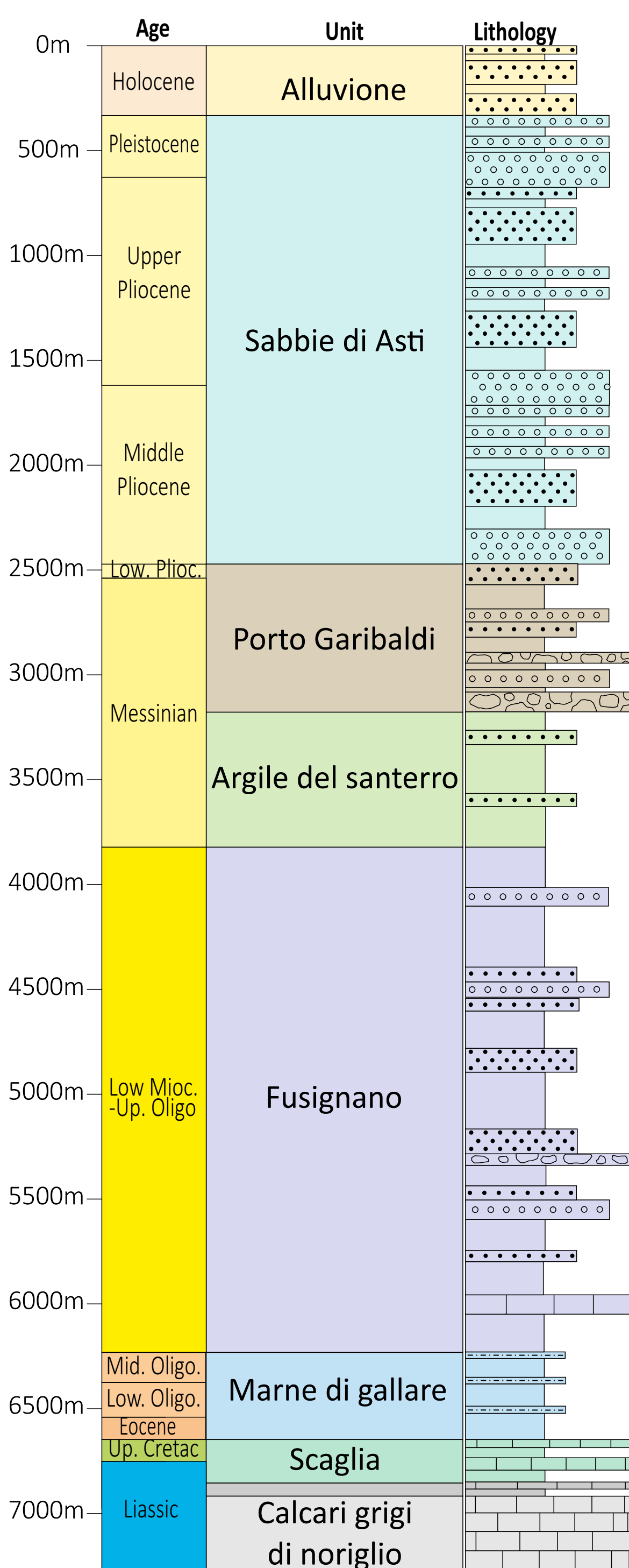
Fig. 4: Stratigraphic column of an example of deep well in the Po basin, based on the reports of the Videpi database.
