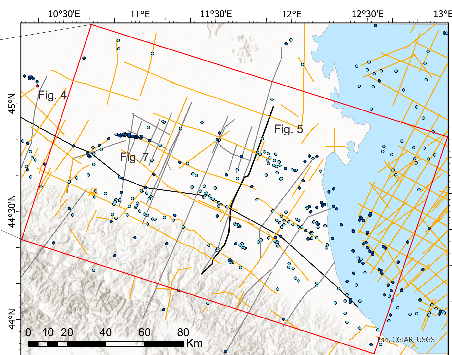
Fig. 3: Study area (limited by red rectangle) with location of the available subsurface information: well reports and logs, 2D seismic lines, and interpreted sections.
